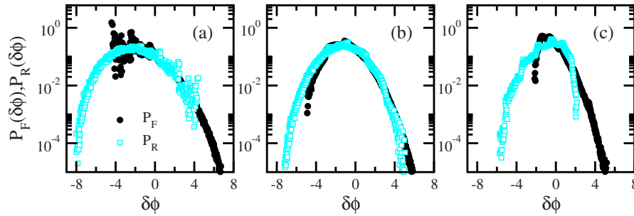
FIG. 2. (Color online) Probability distributions P_F and P_R as a function of \delta\phi for the forward and reversed processes: (a) model 1, (b) model 2, (c) model 3, with \lambda=1 , D=1 , and N=8 . In all cases the rate of particle creation was changed from h_0=0.2 to h_M=1.4 in M=8 steps. The scattering in the data is not due to poor statistics, as we are using a numerical exact method for the computation of the probability distributions.
