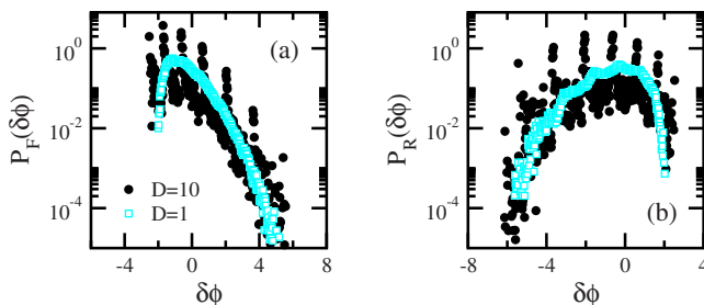
FIG. 3. (Color online) Probability distributions P_F (a) and P_R (b) as a function of \delta\phi for model 3 with \lambda=1 , N=8 , and h changing from h_0=0.2 to h_M=1.4 in M=6 steps. The peaks are more pronounced for larger values of D .
