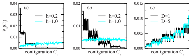
FIG. 1. (Color online) Stationary probability distributions for (a) model 1 with \lambda=1 and D=1 , (b) model 3 with \lambda=1 and D=1 , and (c) model 2 with \lambda=1 and h=1.4 . Shown are the distributions for two values of the creation rate h , respectively, of the diffusion constant D , for systems with N=8 lattice sites. The configurations are grouped by number of particles.
