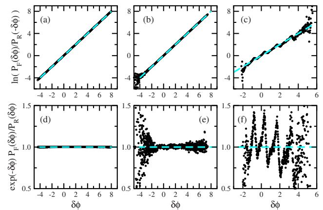
FIG. 4. (Color online) Ratio P_F(\delta\phi)/P_R(-\delta\phi) as a function of \delta\phi for (a) and (d) model 1, (b) and (e) model 2, and (c) and (f) model 3, with \lambda=1 , D=1 , N=8 , and M=8 , whereas h is changed from h_0=0.2 to h_M=1.4 . In the lower panels we plot e^{-\delta\phi}P_F(\delta\phi)/P_R(-\delta\phi) in order to highlight deviations from the equilibrium behavior (3). The dashed lines indicate the expected behavior (3) for a system in equilibrium before and after the change of parameter.
